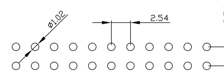
Recommended P.C.B Hole Layout
